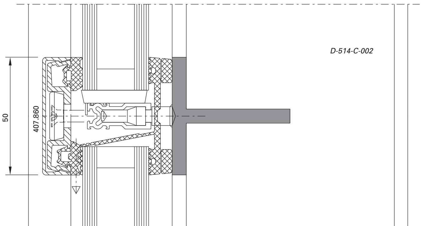
Detail of transom Width 50 mm Welding stud
