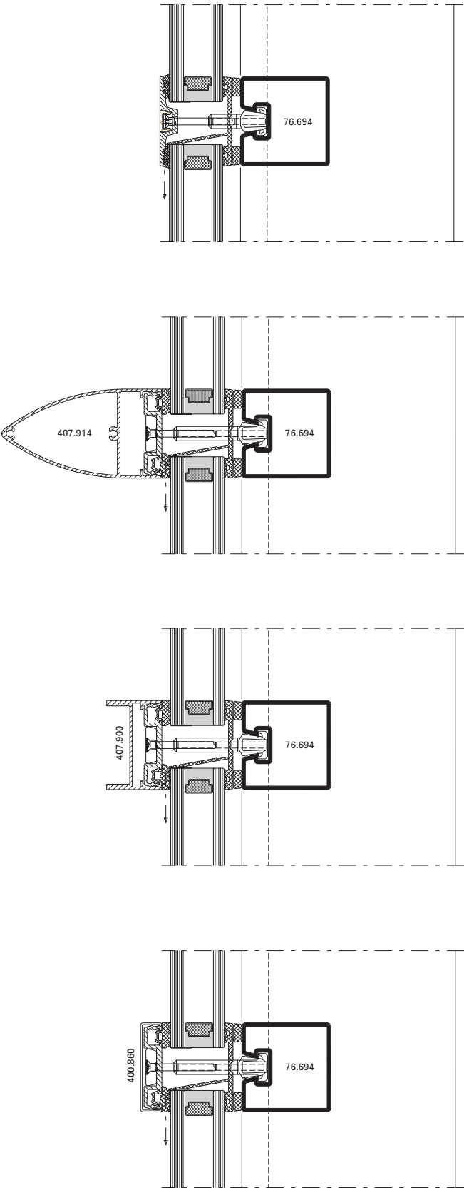
Varianten C-C
