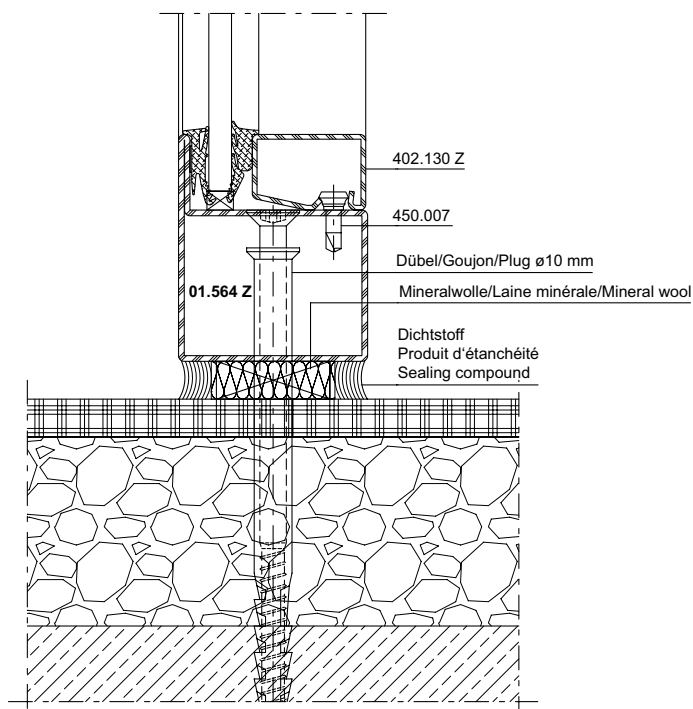
DXF DWG 41-0102-A-037
