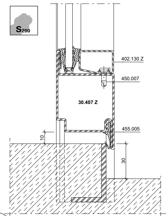
DXF DWG 41-0102-A-056
