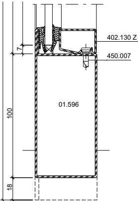
Detail E
