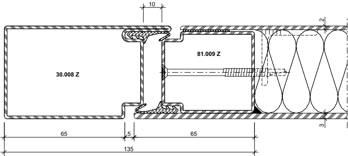
DXF DWG 41-0103-C-023
