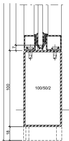
Detail E
