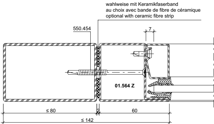
DXF DWG 41-0102-K-059
