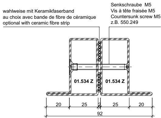
DXF DWG 41-0102-K-021
