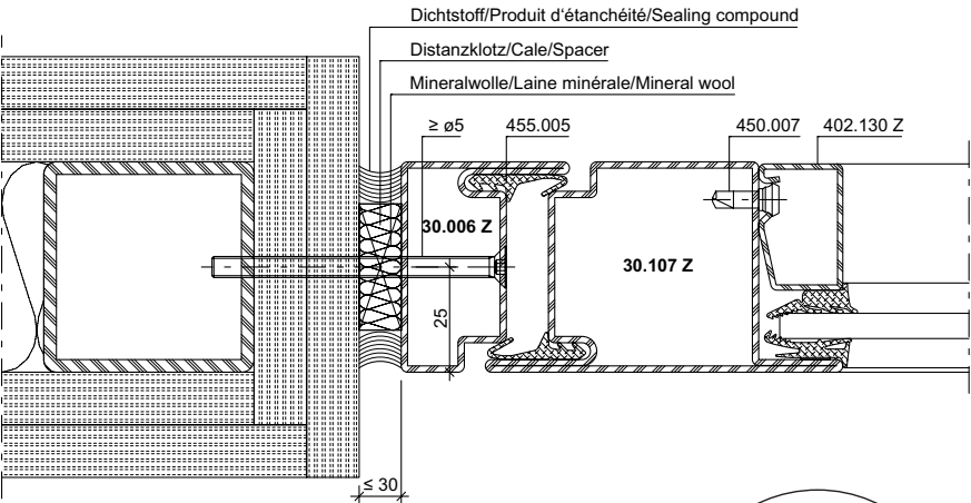
DXF DWG 41-0102-A-099
