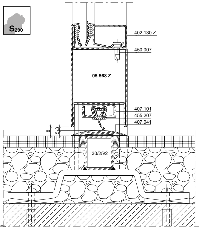
DXF DWG 41-0102-A-023
