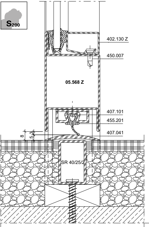
DXF DWG 41-0102-A-040
