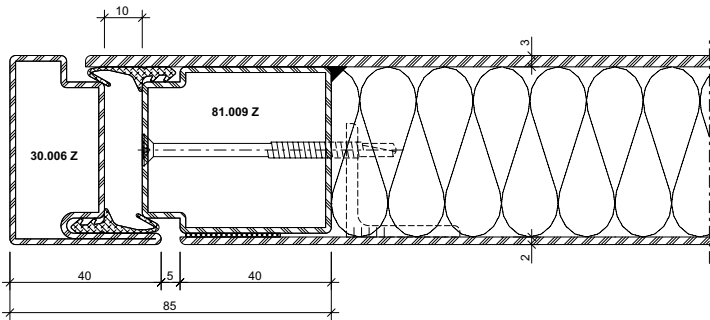
DXF DWG 41-0103-C-025
