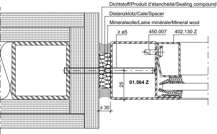
DXF DWG 41-0102-A-079
