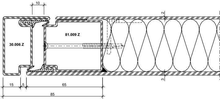
DXF DWG 41-0103-C-026
