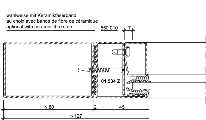
DXF DWG 41-0102-K-060
