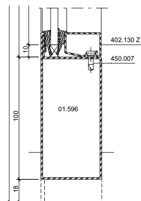
Detail E
