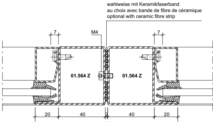
DXF DWG 41-0102-K-003
