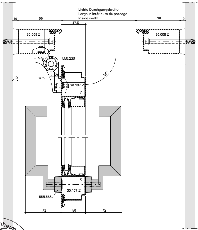
DXF DWG 41-0101-E-006
