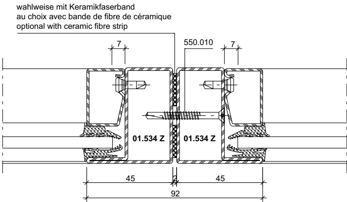
DXF DWG 41-0102-K-002
