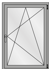
Drehkipp-Flügel Vantail oscillo-battant Turn/tilt window
