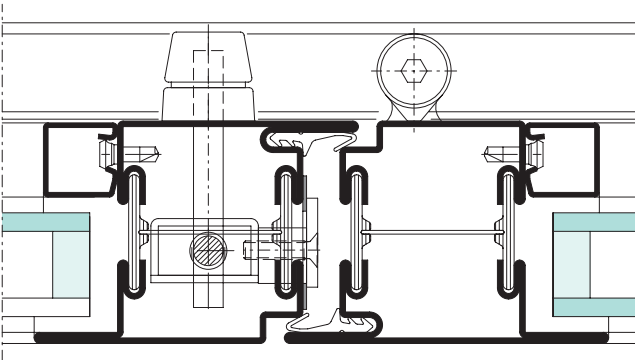
Section detail
