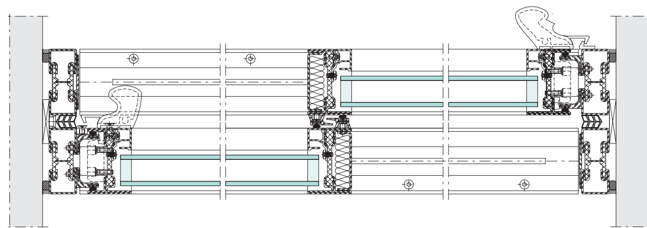
Section detail
