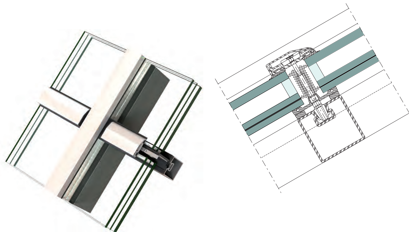
Section detail
