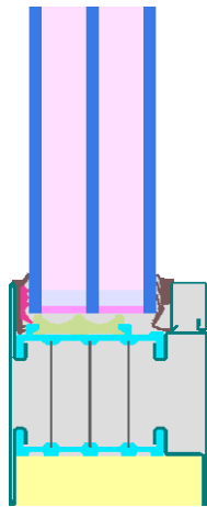
Calculation model
