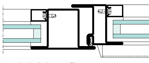
Standard window profiles
